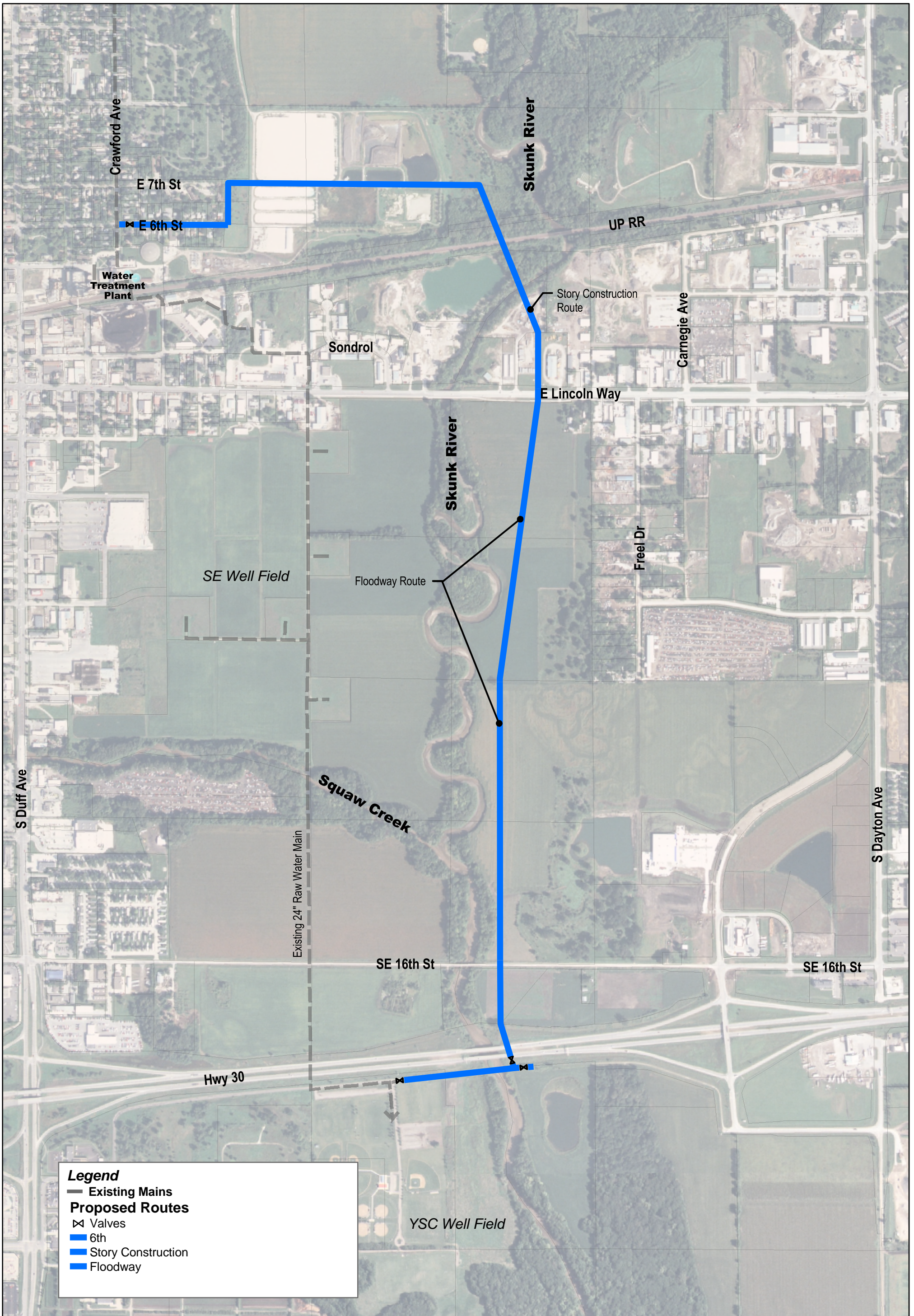
FIGURE 2: Selected Route Raw Well Water Transmission Pipeline Water & Pollution Control Department Ames, Iowa
